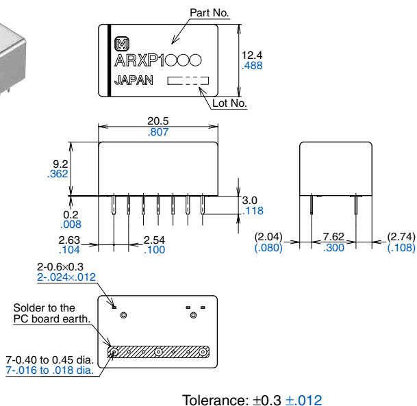
External dimensions
